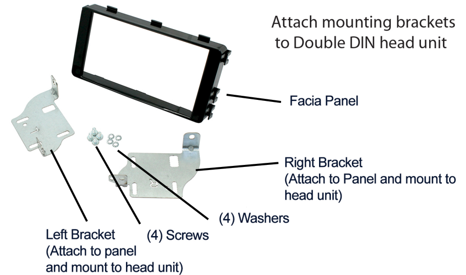
6. Attach facia plate to mounting brackets and fix it
