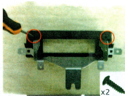
7 Take the bracket previously fixed and fix it on the aftermarket radio unit with the supplied screws (choose the appropriate type of screw between the two types supplied, see the picture below) on each side of the radio. See the picture to check the position of the screws.
