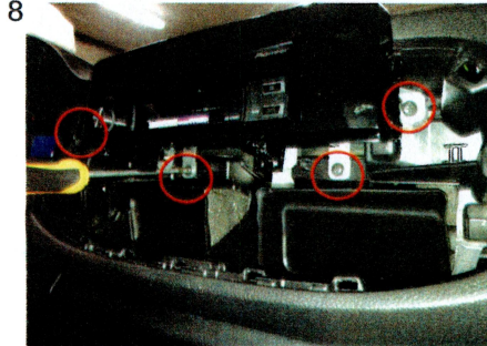
8 Connect all cables, verify the proper functioning of the system and insert the unit into the radio tunnel. Fix it with the screws saved and the bolt before as shown in the pictures.
